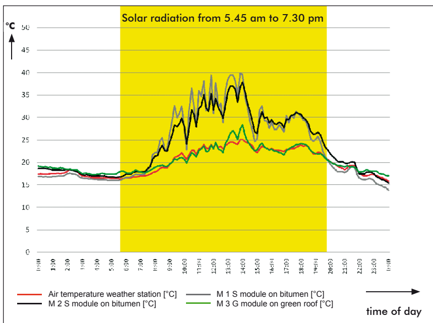
Graph: example of temperature graph recorded on a day in July. The temperature of the modules on the bituminous panels (black and grey lines) rises to almost 40 °C, while that of the module on the green roof (green line) does not go beyond a maximum of 27 °C and is, therefore, close to the ambient temperature (red line).
