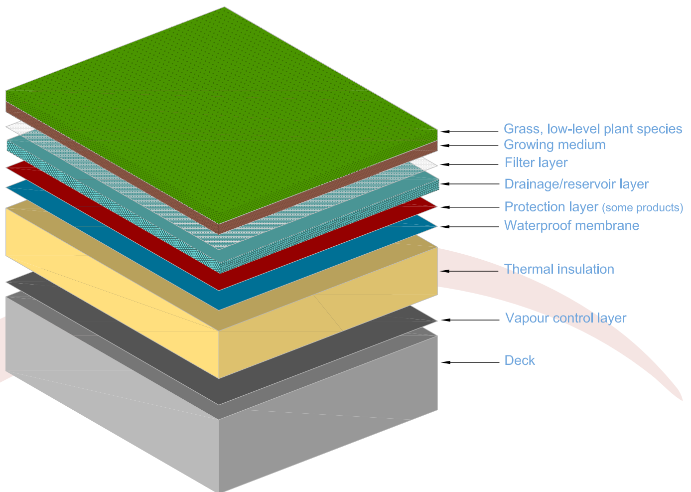
Fig. 3 Green roof - (Warm roof type) (section)
