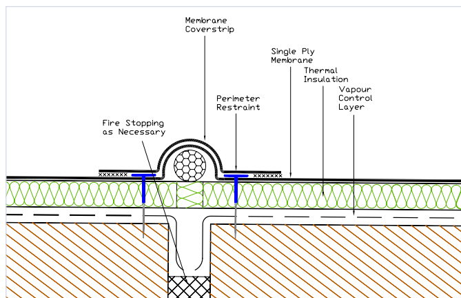
Detail 3 Movement joint – waterproof - principles
