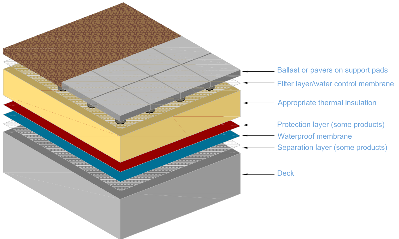
Fig. 2 Inverted warm roof (section)
