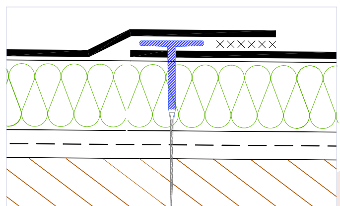
Fig.5 Mechanical fastening – in-seam fastening of membrane
