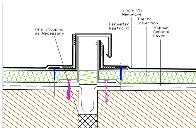
Detail 4 Movement joint – weatherproof - principles
