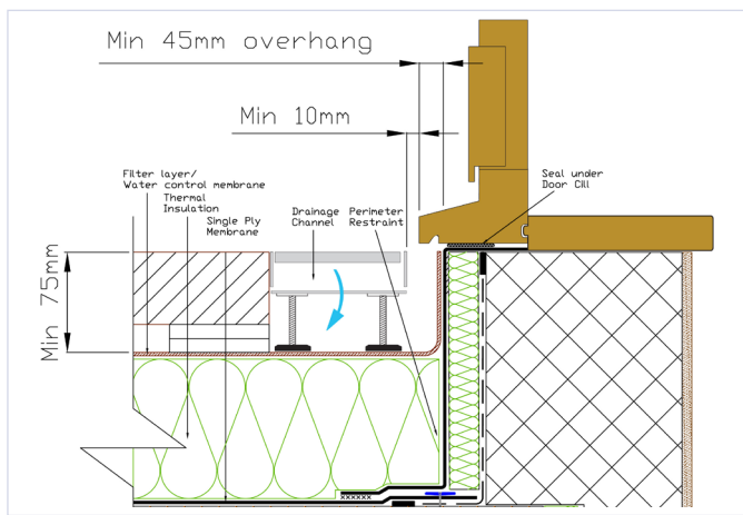
Detail 7 Level threshold – inverted warm roof - principles
