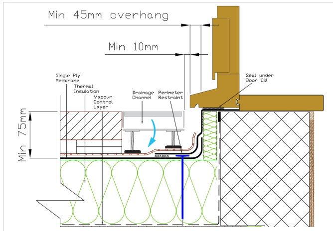
Detail 6 Level threshold – warm roof – principles
