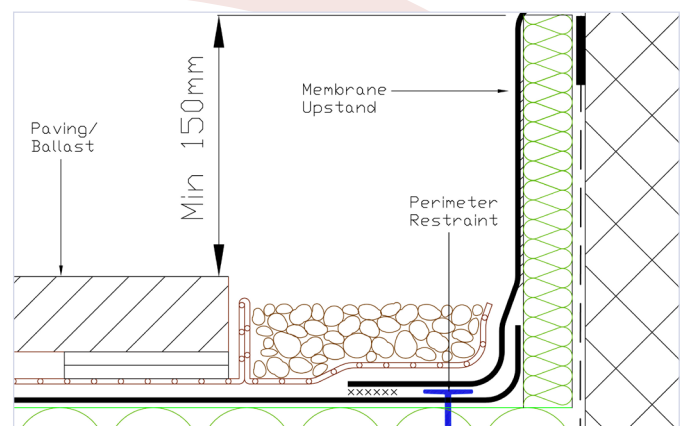
Detail 1 Upstand – minimum height
