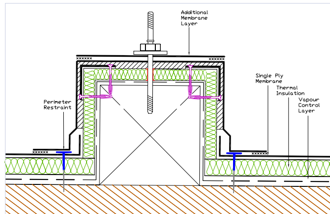
Detail 5 Load-bearing plinth for plant - principles
