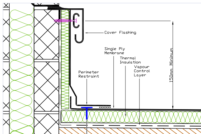
Detail 2 Weatherproof upstand - principles
