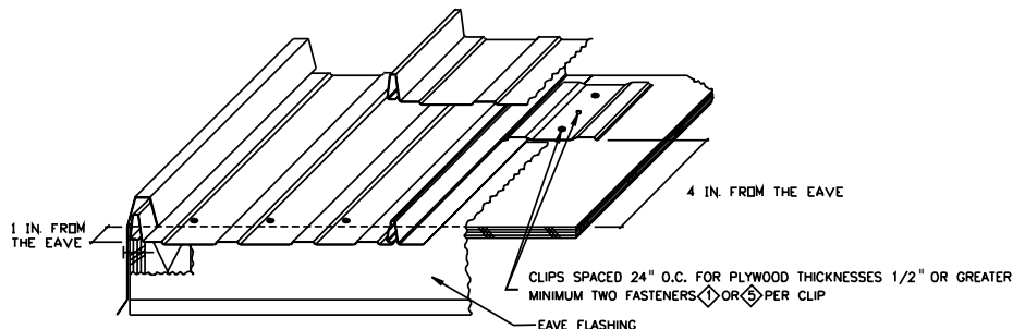
16" Panel Shown
